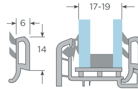
Junquillo termopanel 17-19mm Andes
