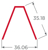
Ref. esquinero 45° 1.5mm RF351535
