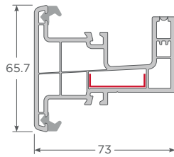
Divisor marco corredera monoriel
