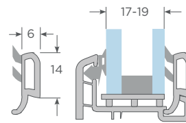
Junquillo termopanel 17-19mm
