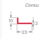
Ref. Contra Flecha 2mm - TC PL-CMP-TC-CTF-2
