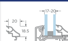
Junquillo 17-20mm S60
