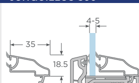
Junquillo 4-5mm S60
