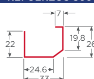
Ref. New Múltiple 1.2mm - TC PL-CMP-TC-MLT-12
