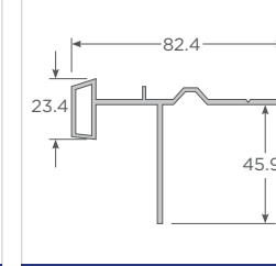
New Aleta Siding
