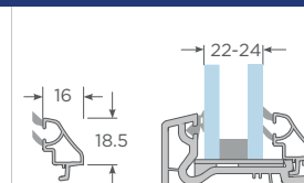
Junquillo 22-24mm S60
