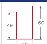
Ref. Hoja Puerta S60 1.5mm - TC PL-S60-TC-HPF-15
