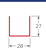
Ref. Poste T S60 1.2mm - TC PL-S60-TC-PST-12
