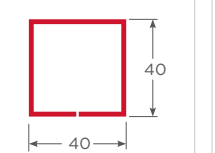
Ref. Box esquinero 90° S60 1.5mm - TC PL-S60-TC-EQF-15
