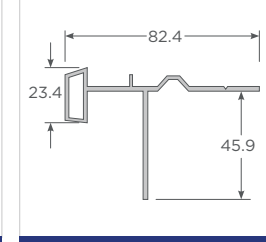
New Aleta Siding
