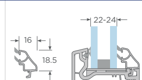
Junquillo 22-24mm S60
