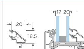
Junquillo 17-20mm S60
