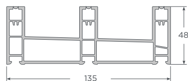
Marco Triple Riel Corredera S75
