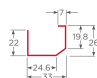
Ref. New Múltiple 1.2mm - TC PL-CMP-TC-MLT-12
