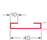
Ref. Marco Sliding Múltiple 1.2mm - TC PL-SLD-TC-MLT-12
