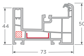
Marco Monorriel Corredera Andes
